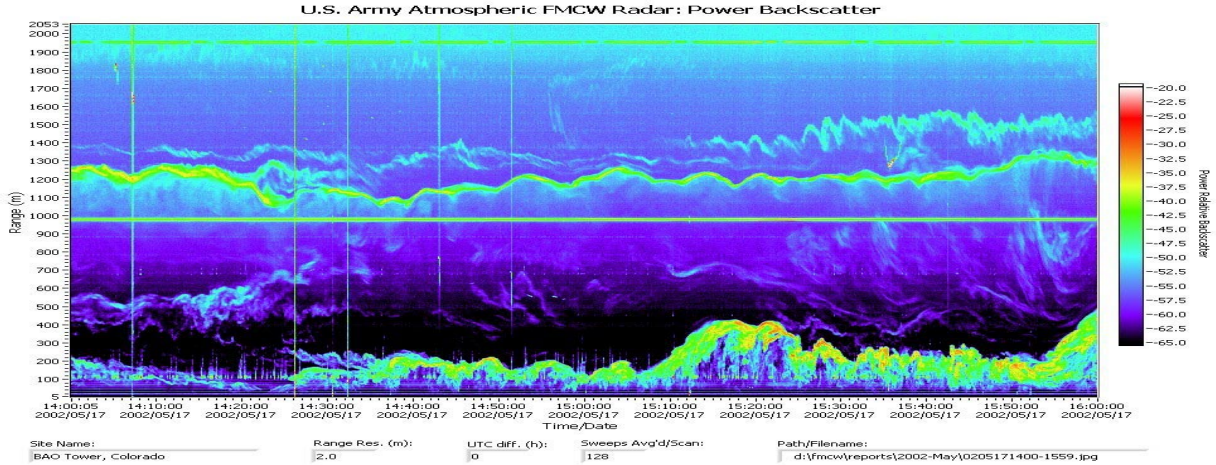
Figure 4 Clear-air turbulence as seen by the FM-CW radar. Two hours of data with 2-meter resolution, from near ground to 2050 meters, May 17, 2002, Erie CO).
