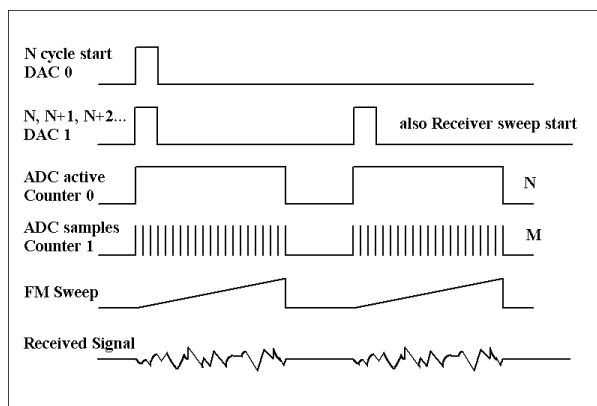
Figure 3 Basic FM-CW radar control and timing.
