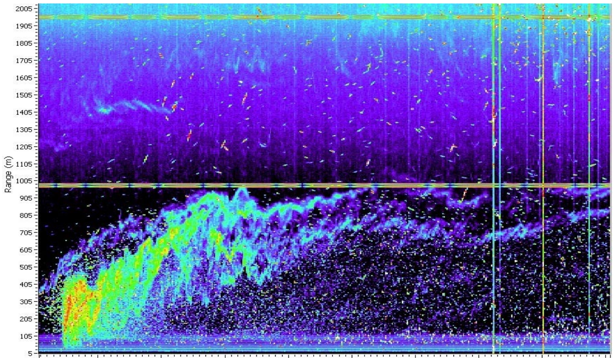
Figure 9 Apparent frontal signature and insects as seen by U.S. Army FM-CW radar at Dugway Proving Ground, UT. (0-2105 meters, 2 meter resolution, 1 hour of data left-to-right, early evening, Fall 2001)
