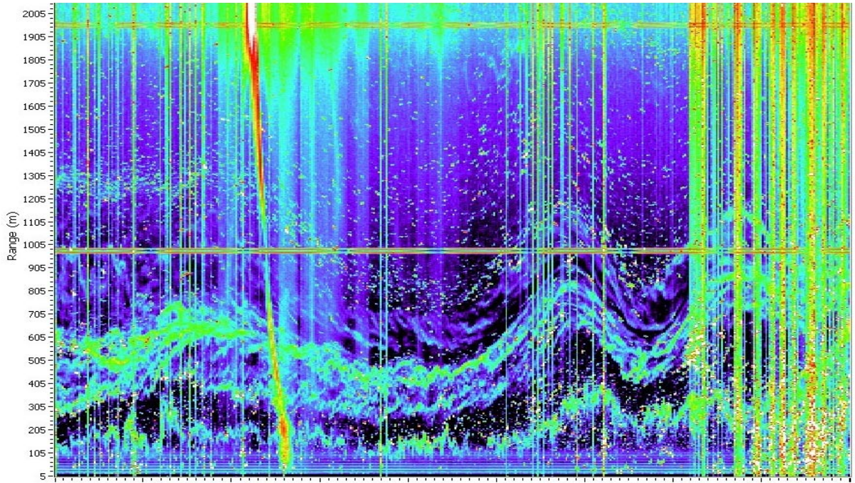
Figure 8 Clear-air wave structures, brief rain, insects and birds, as observed by the Army FM-CW radar at Dugway Proving Ground, UT. (0-2105 meters, 2 meter resolution, 1 hour of data left-to-right), mid-morning, early Fall 2001)
