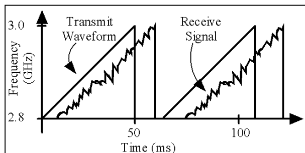
Figure 2 FM-CW Tx and Rx waveform
