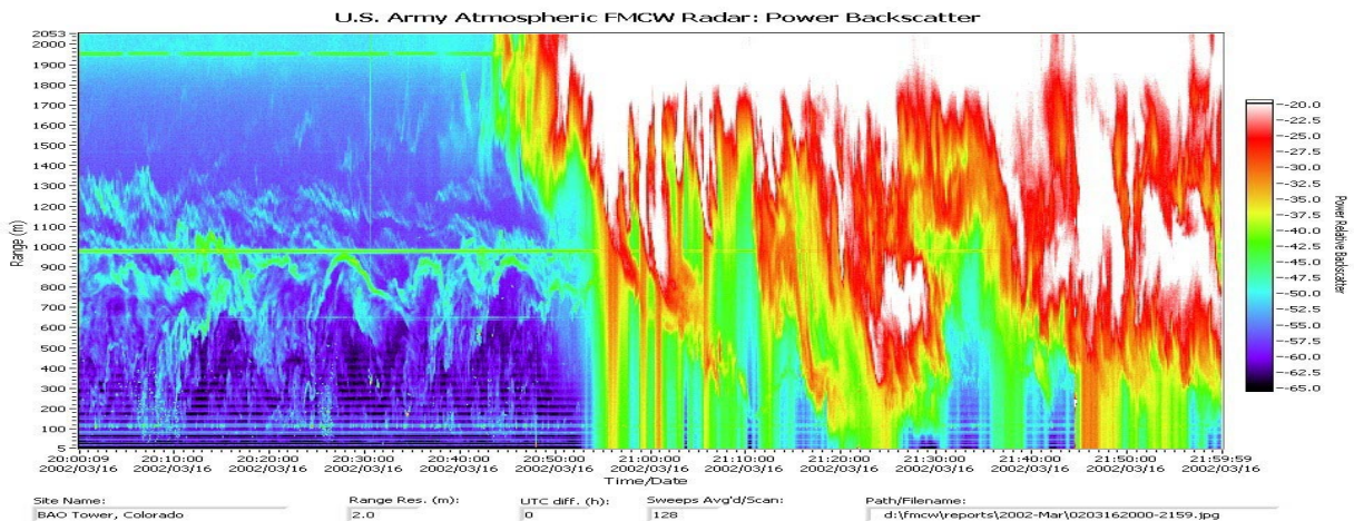
Figure 5 Clear-air turbulence and rain. Horizontal streaks are interference from TWT. (0-2053 meters AGL, 2 hours left-to-right, March 16, 2002 Erie CO)
