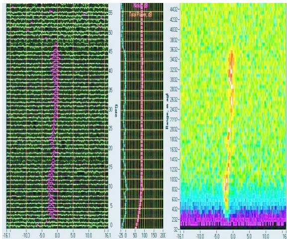
Illustration 6. Stacked spectra display of the Dwell software
