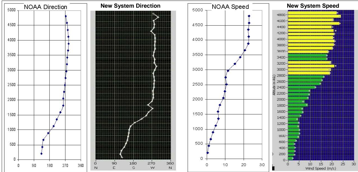
Illustration 8. NOAA 449 MHz Platteville data and New 449 MHz System data for May 15, 2004, 1700 UTC. In order from left to right: NOAA wind direction, New System wind direction, NOAA wind speed, New System wind speed. Note that the NOAA profiler data is for an entire hour average while the New System provides data for a 10 minute average. The systems are about 20 km apart.
