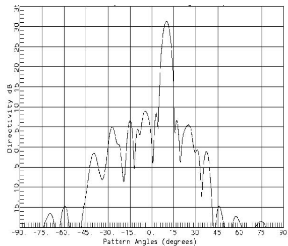
Illustration 3. Example calculated antenna array radiation pattern cut, showing low sidelobes.
