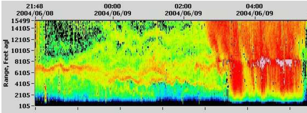
Illustration 9. Range-corrected 0th (power) moment data. The low signal values in the lowest gates are due to the STC. While not shown here, the 1st moment data is still available and is used for the wind calculation.
